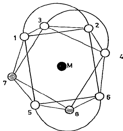
Fig. 1. Structure of [\text{Ln}(\text{acac})_3(\text{H}_2\text{O})_2] unit showing \equiv \text{H}_2\text{O} molecules and \circ oxygen.
