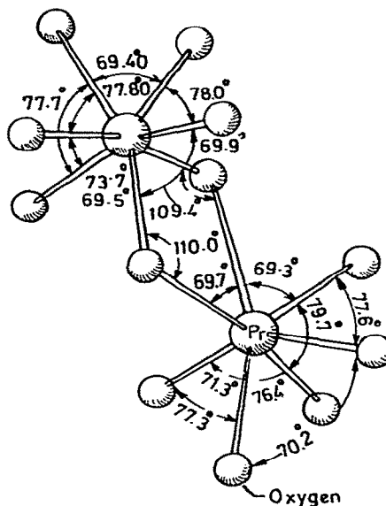
Fig. 1. Structure of [\text{Ln}(\text{acac})_3(\text{H}_2\text{O})_2] unit showing \equiv \text{H}_2\text{O} molecules and \circ oxygen.
